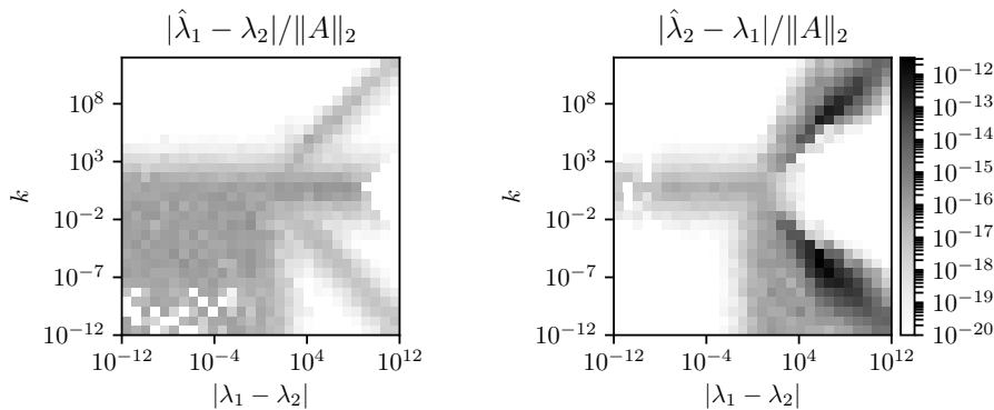
FIG. 4. Relative forward error on the eigenvalues after the swap computed with the QR update.
