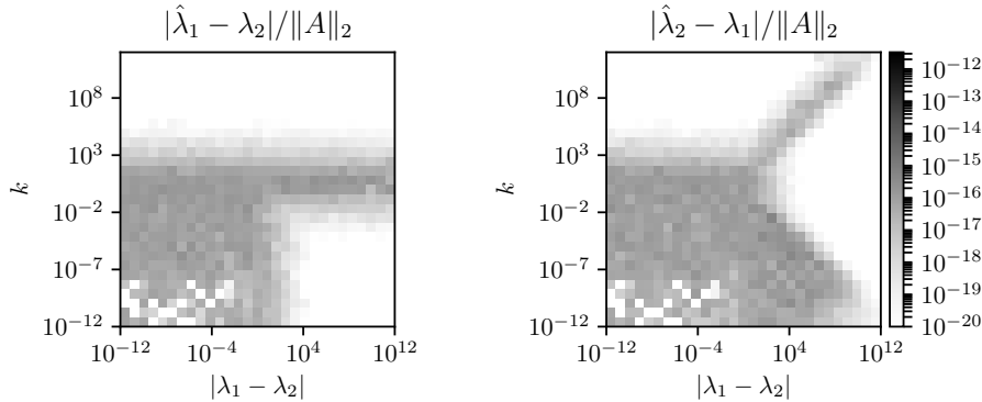
FIG. 3. Relative forward error on the eigenvalues after the swap computed with the SVD update.
