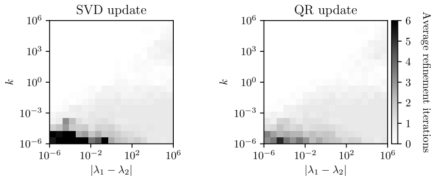
FIG. 5. Average number of iterative refinement iterations.
