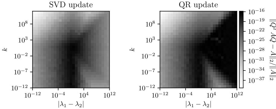
FIG. 2. Relative backward error of the swap.
