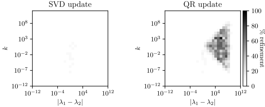
FIG. 1. Percentage of times the swap required iterative refinement.
